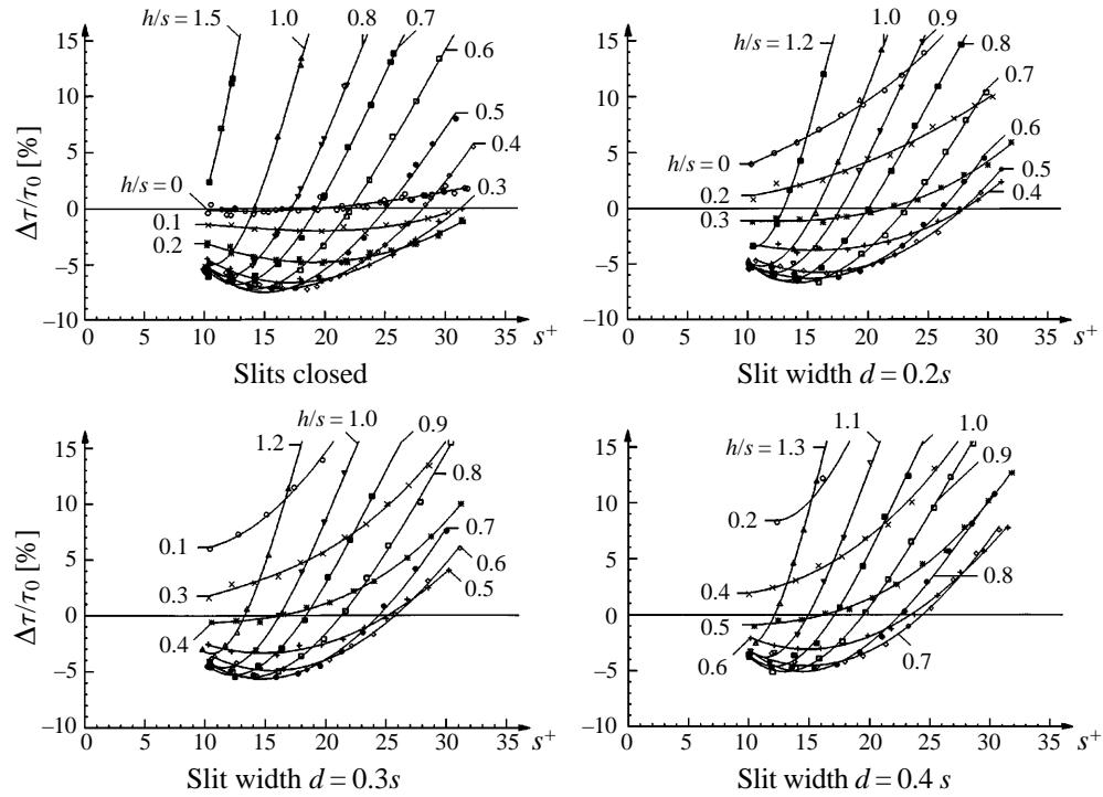
FIGURE 12. Shear stress data of the plate with slits and longitudinal blades.
