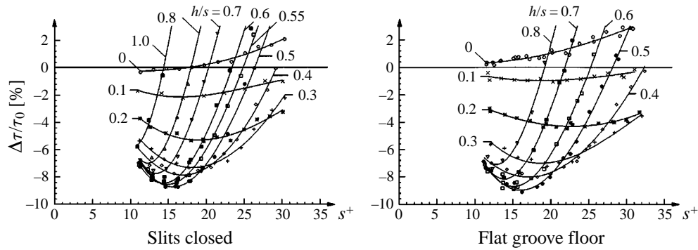
FIGURE 13. Optimization of blade riblets, decreased blade thickness t = 0.01s .
