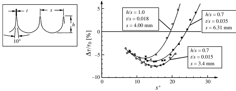
FIGURE 9. Scalloped riblets with increased groove depth.
