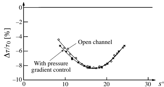
FIGURE 23. Influence of shear stress distribution on drag reduction data.
